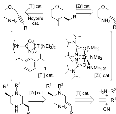
Scheme 1. Hydroamination with N,O-chelated group 4 precatalysts for the synthesis of 3-substituted morpholines and 2,5-substituted piperazines. Noyori's cat. = [( S,S )-Ts-dpen]( p -cymene)RuCl].
