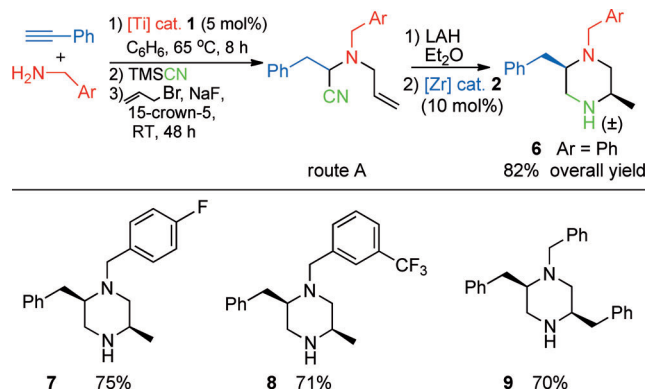
Scheme 4. Modular, diastereoselective synthesis of 2,5-disubstituted piperazines from commercially available starting materials. Yields shown are overall yields of isolated product using alkyne as the limiting reagent. LAH = lithium aluminum hydride, TMS = trimethylsilyl.
