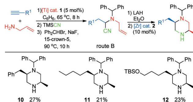
Scheme 5. Flexible, modular, diastereoselective synthesis of N -benzhydryl substituted 2,5-disubstituted piperazines from commercially available starting materials. Yields shown are overall yields of isolated product using alkyne as the limiting reagent. LAH = lithium aluminum hydride, TBS = tert -butyldimethylsilyl, TMS = trimethylsilyl.
